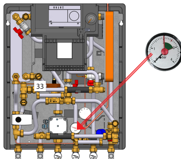
Fig. 1. Akva Lux II VXe, Standard model
